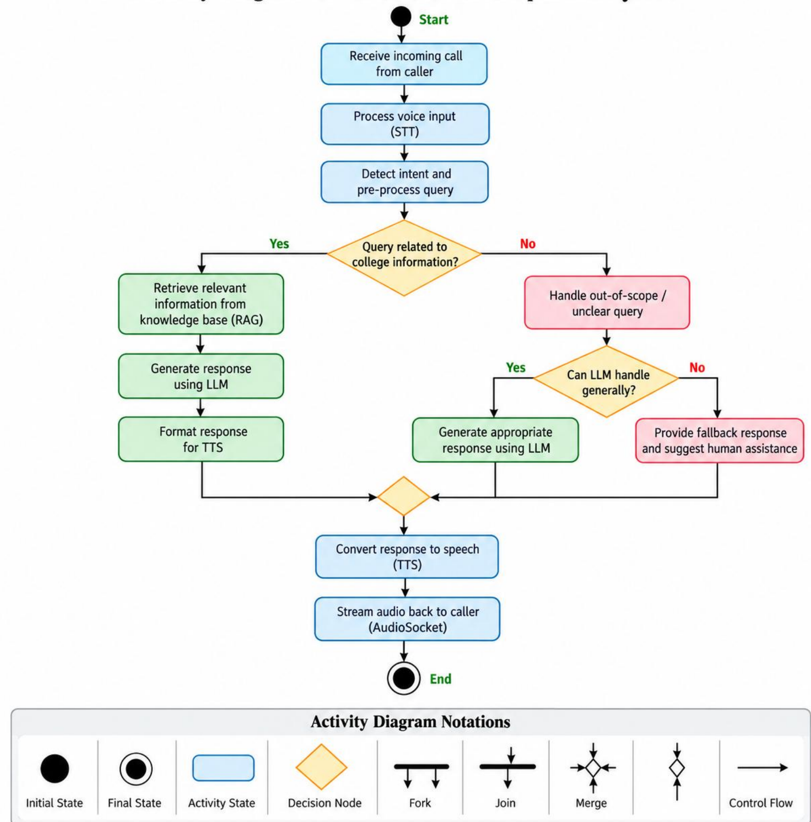
Activity Diagram for Voice-Based AI Receptionist System
